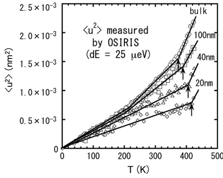
FIG. 1. Temperature dependence of mean-square displacement \langle u^2 \rangle evaluated in INS measurements by OSIRIS with energy resolution of 25 \mu\text{eV} for aPS bulk, 100, 40, and 20 nm films.
